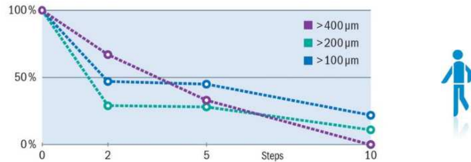
Fraunhofer IPA test results for shoe-soles
