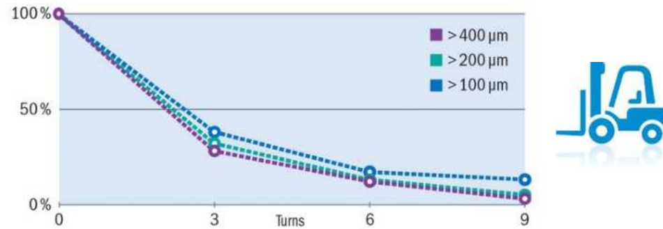
Fraunhofer IPA test results for forklift truck tires
